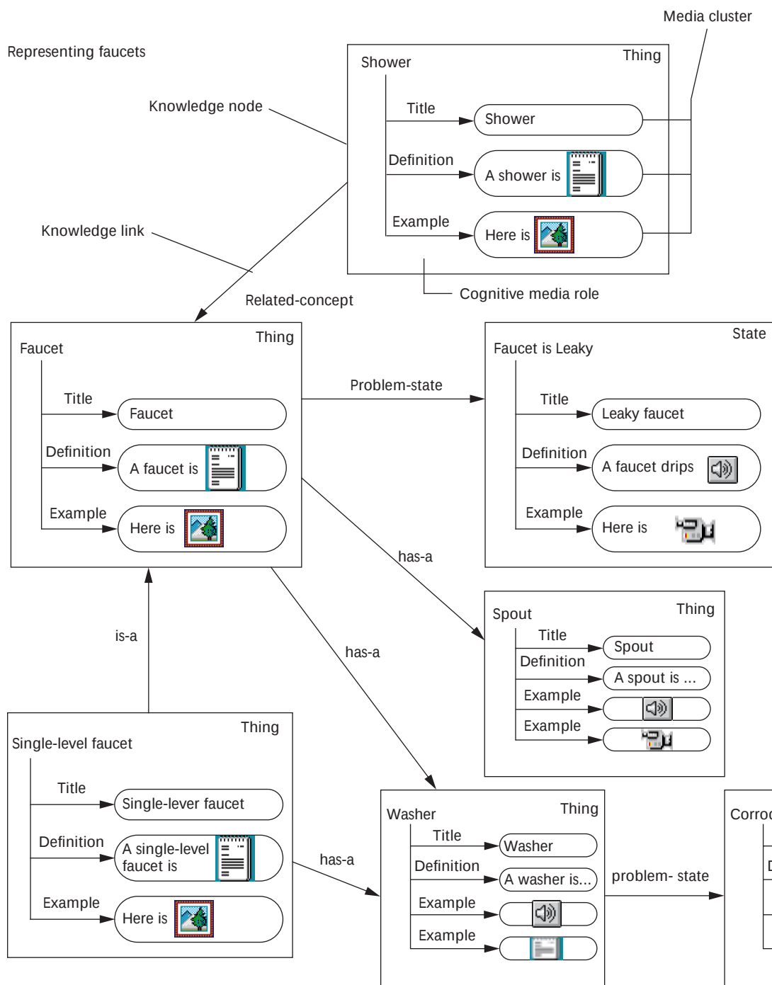
Figure 2. A PML knowledge structure about faucets.
