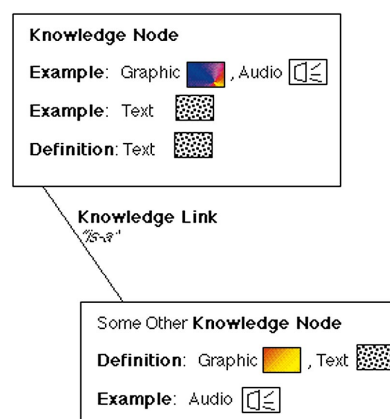
Figure 1. Knowledge representation in PML. Definition and Example are cognitive media roles and can have more than one associated physical media cluster, such as Audio and Graphic.
