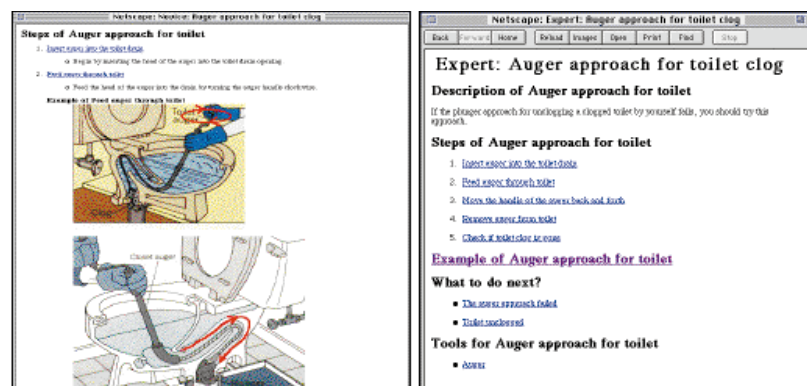
Figure 7. Two presentations based on the same PML source. (a) The presentation aimed at the novice offers detailed explanations and examples; (b) The one for an expert is more concise, but with links to further explanations.
